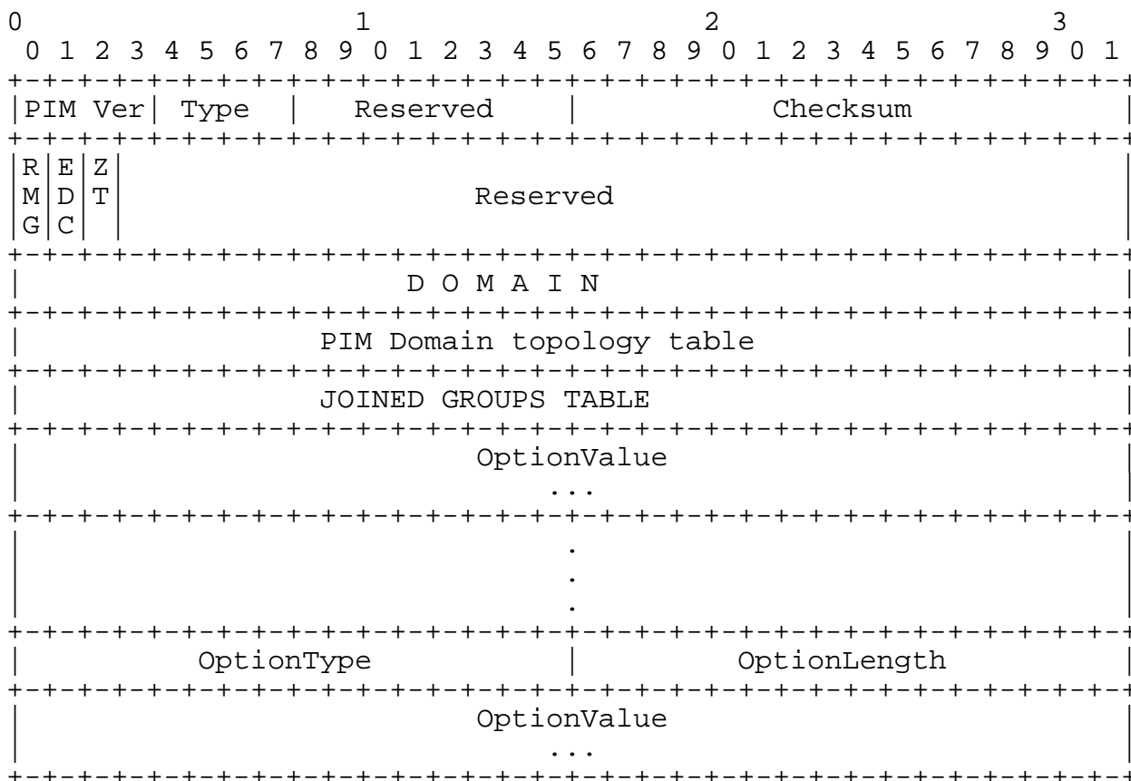
Figure 15 original PIM-SM hello packet compared with the new hello packet format
